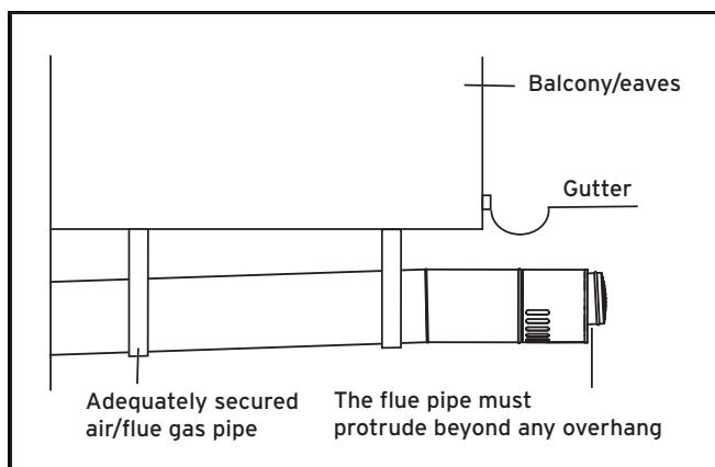
Horizontal Termination
